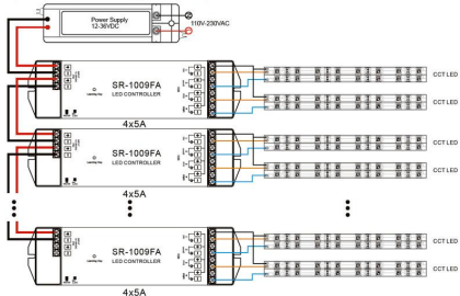
2) Receiver Connection Diagram for Multiple Units
